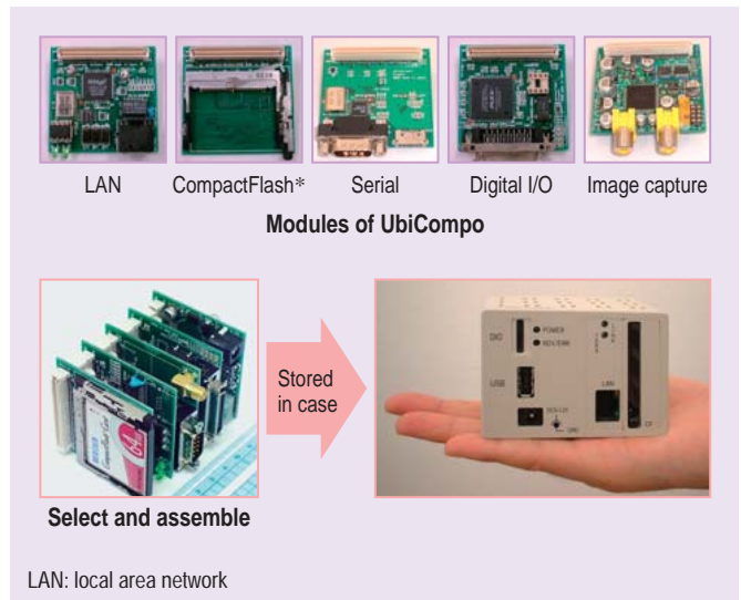
Modules and architecture of ultra-small ubiquitous controllers "UbiCompo"
