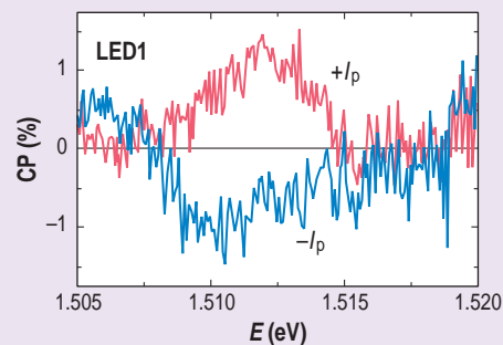
(a) Polarization along z axis measured with active LED1 for two opposite I_p directions
