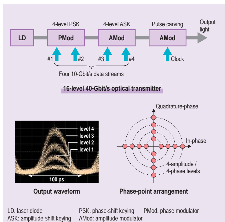
16-level 40-Gbit/s optical modulation
