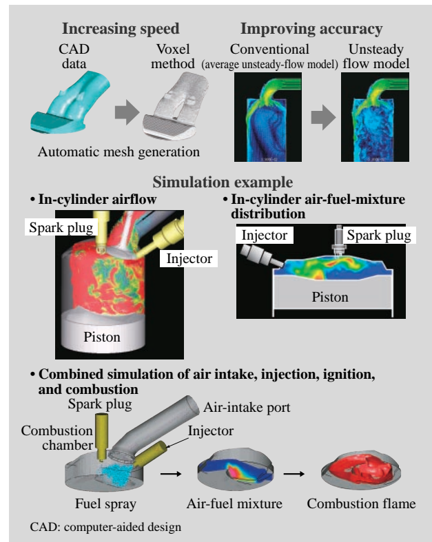
Fig. 5—Simulation and Analysis Technology. The engine-combustion simulation technique achieves high-speed mesh generation by the voxel method and accuracy improvement by modeling of unsteady flow. Based on this analysis technique, specifications of product components and combustion concepts are being proposed.
