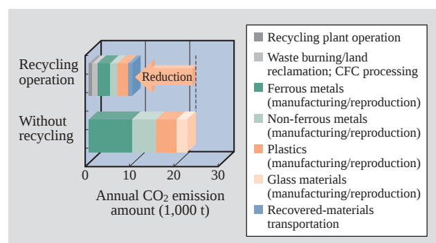
Fig. 8—Effect of Reducing CO 2 Emissions by Recycling Household Appliances.
