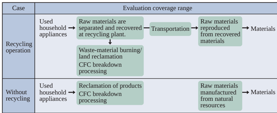
Fig. 7—Method for Evaluating Effects of CO 2 Emission Reduction by Recycling.
