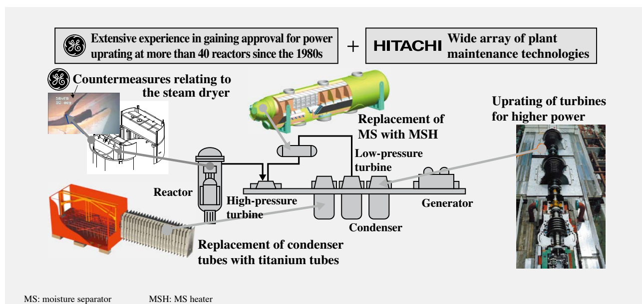
Fig. 3—Technologies for Increasing Power Output.
