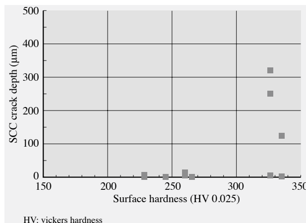
Fig. 4—Relationship between SCC Crack Depth and Surface Hardness.
